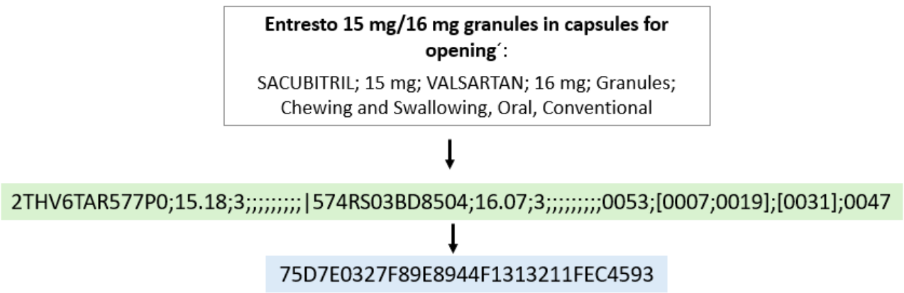
Figure 6. An example on multiple AME and two substances as input in PhPID.
